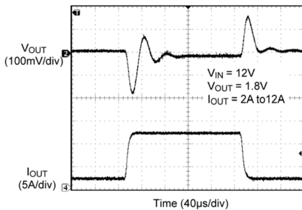
Transient Response
