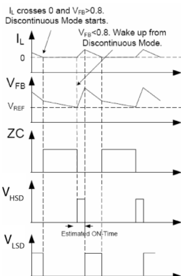
Figure 4. MIC261203 Control Loop Timing (Discontinuous Mode)
