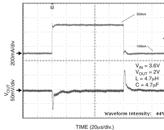
Load Transient
