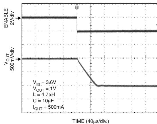
Disable Transient
