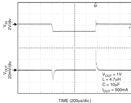
Line Transient
