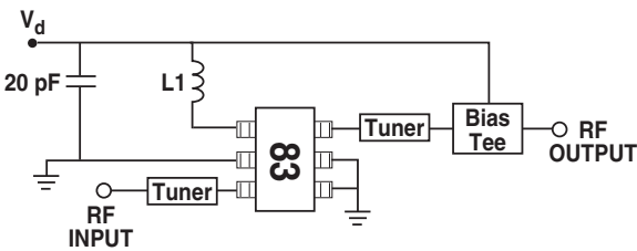
Figure 2. MGA-83563 Test Circuit for Characterization.
