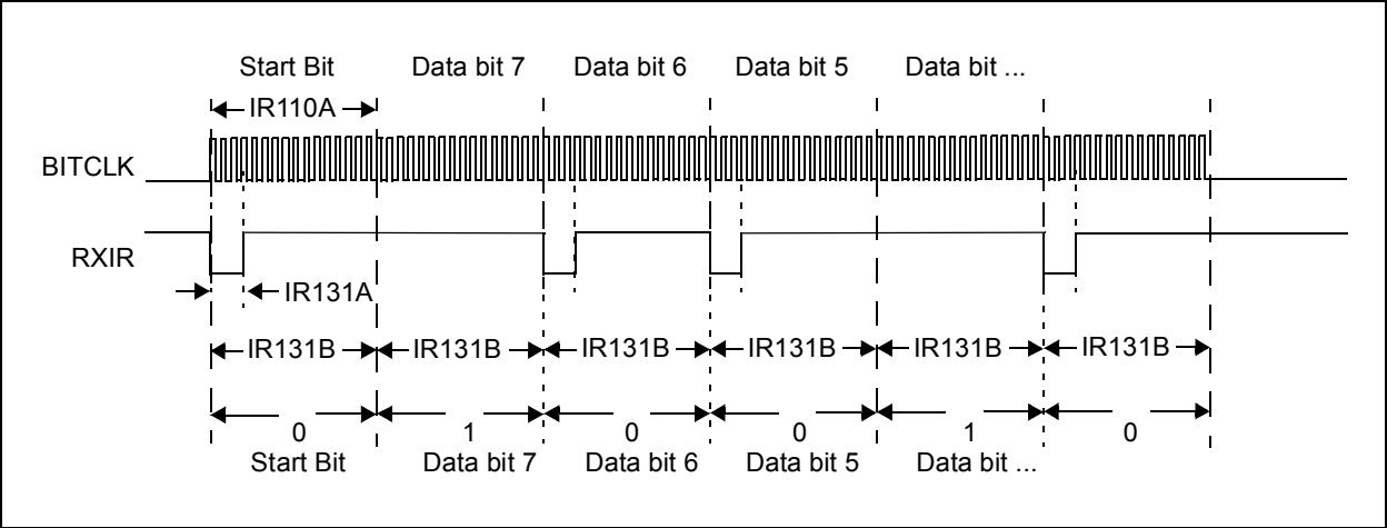
FIGURE 4-9: RXIR WAVEFORMS
