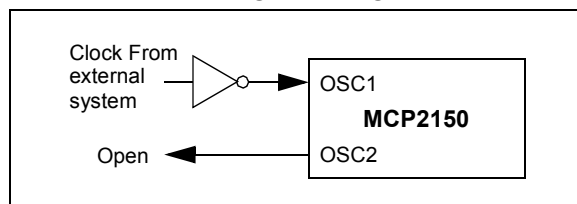
FIGURE 2-2: EXTERNAL CLOCK INPUT OPERATION
