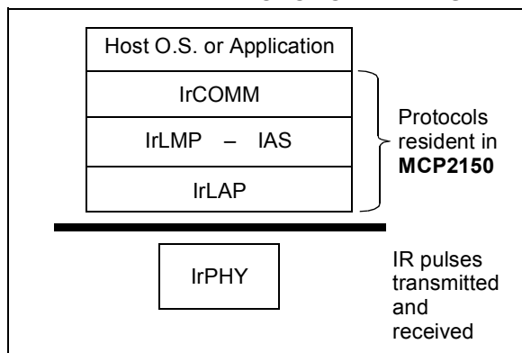
FIGURE 2-7: IRDA STANDARD PROTOCOL LAYERS
