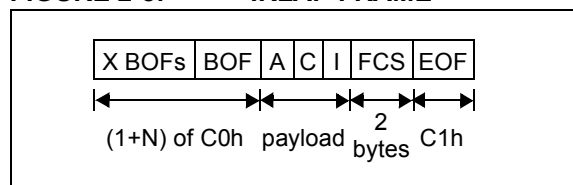
FIGURE 2-8: IRLAP FRAME
