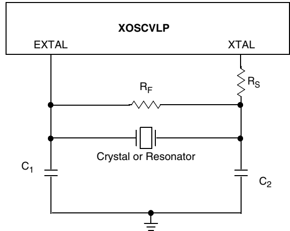
Figure 12. Typical Crystal or Resonator Circuit: High Range and Low Range/High Gain
