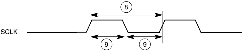
Figure 44. SPI SCLK Timing Diagram
