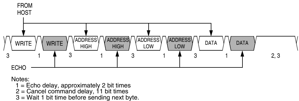
Figure 15-16. Write Transaction
