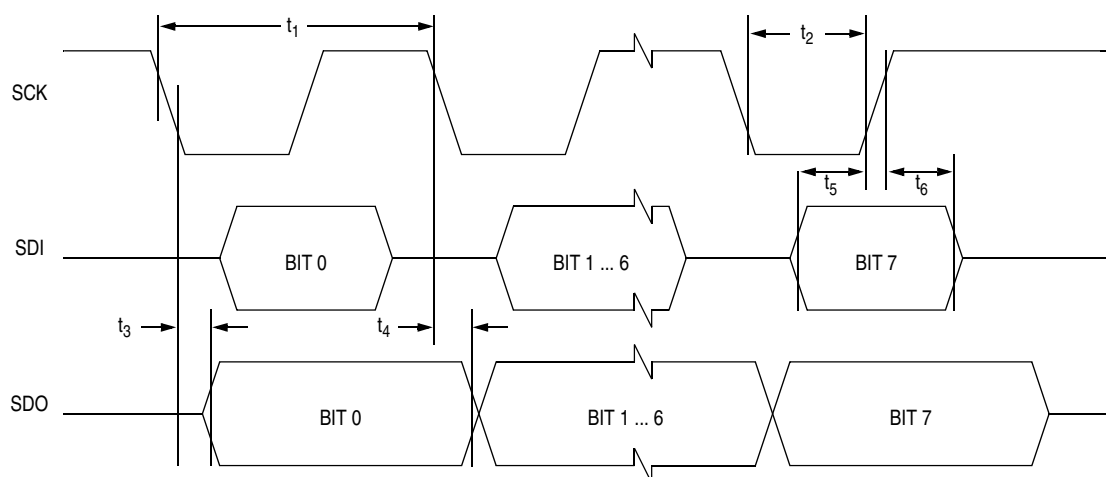
Figure 14-1. SIOPTiming Diagram
