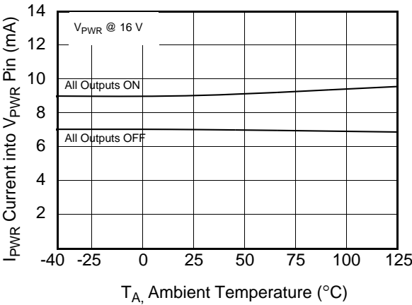
Figure 12. I_{PWR} vs. Temperature
