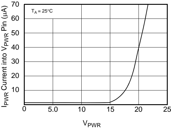
Figure 14. Sleep State I_{PWR} vs. V_{PWR}
