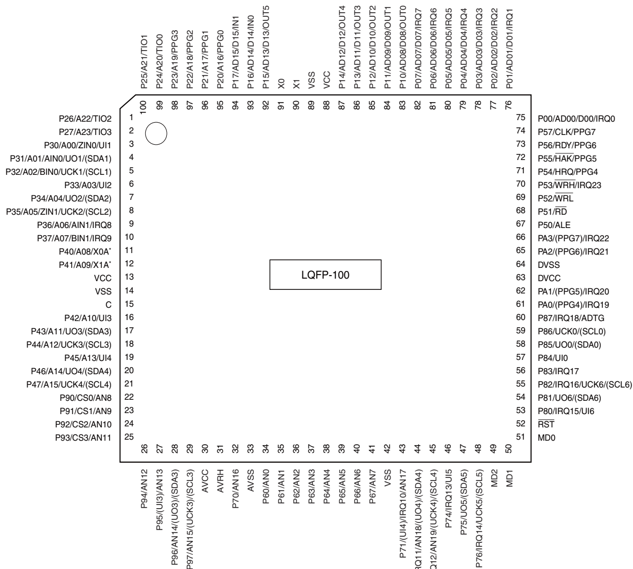
(TOP VIEW)
