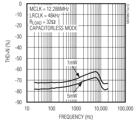
TOTAL HARMONIC DISTORTION + NOISE vs. FREQUENCY (DAC TO HEADPHONE)
