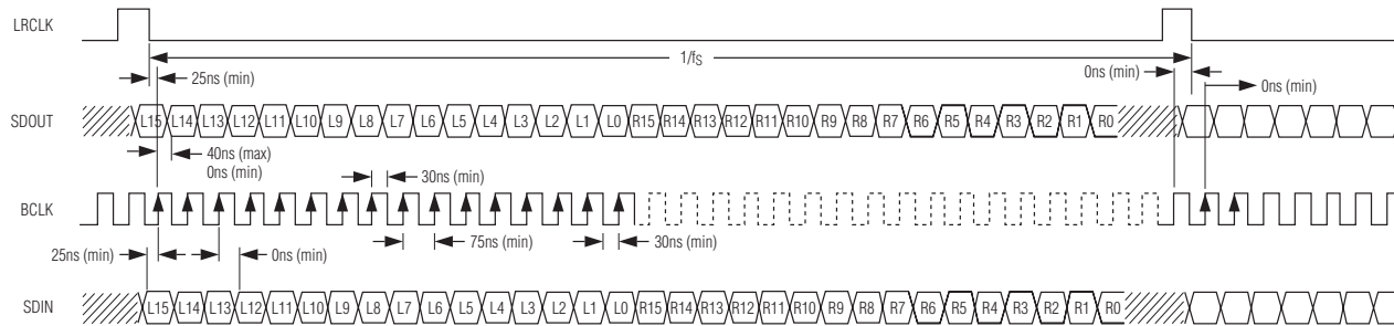
Figure 4. Digital Audio Interface Voice Slave Mode Examples
