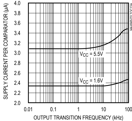
SUPPLY CURRENT PER COMPARATOR vs. OUTPUT TRANSITION FREQUENCY
