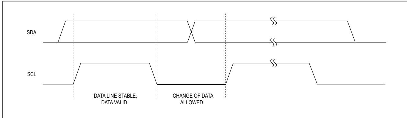
Figure 30. Bit Transfer
