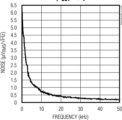
NOISE vs. FREQUENCY ( V_{OUT} = 3V )
