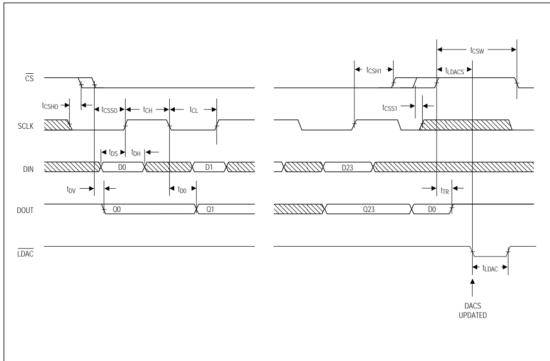
Figure 1. Timing Diagram
