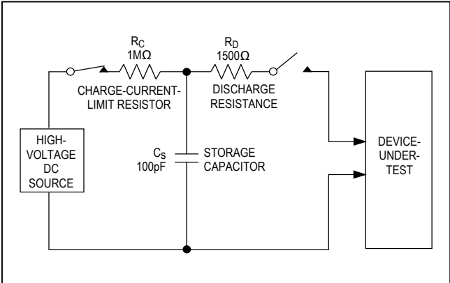
Figure 4a. Human Body ESD Test Model
