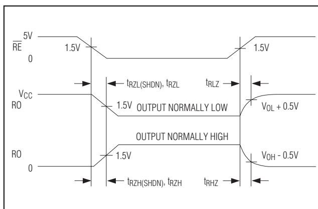
Figure 12. Receiver Enable and Disable Times (Except MAX3081E/MAX3084E/MAX3087E)
