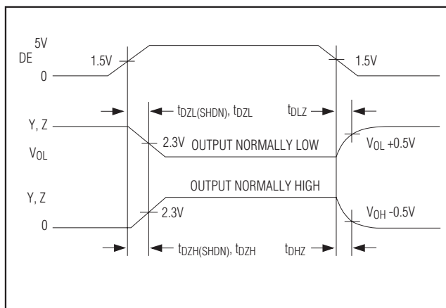
Figure 10. Driver Enable and Disable Times (Except MAX3081E/MAX3084E/MAX3087E)
