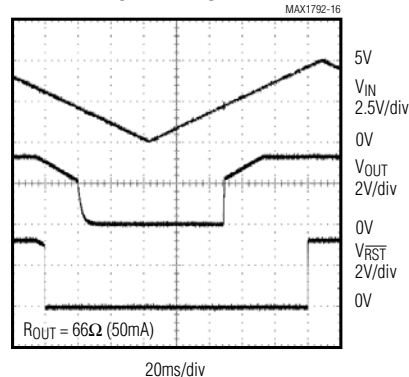
RST WAVEFORM
