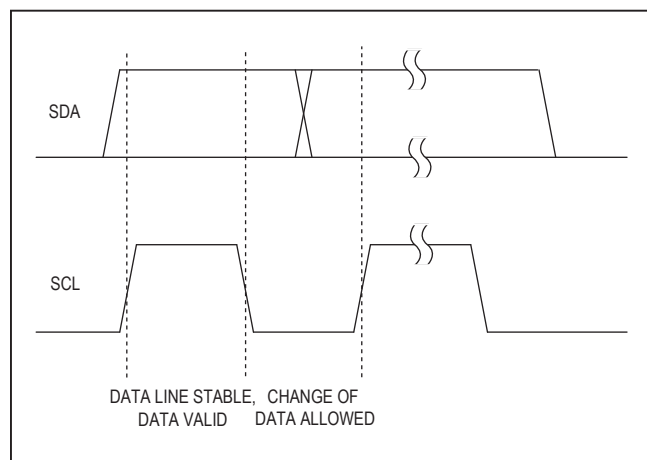
Figure 9. Bit Transfer
