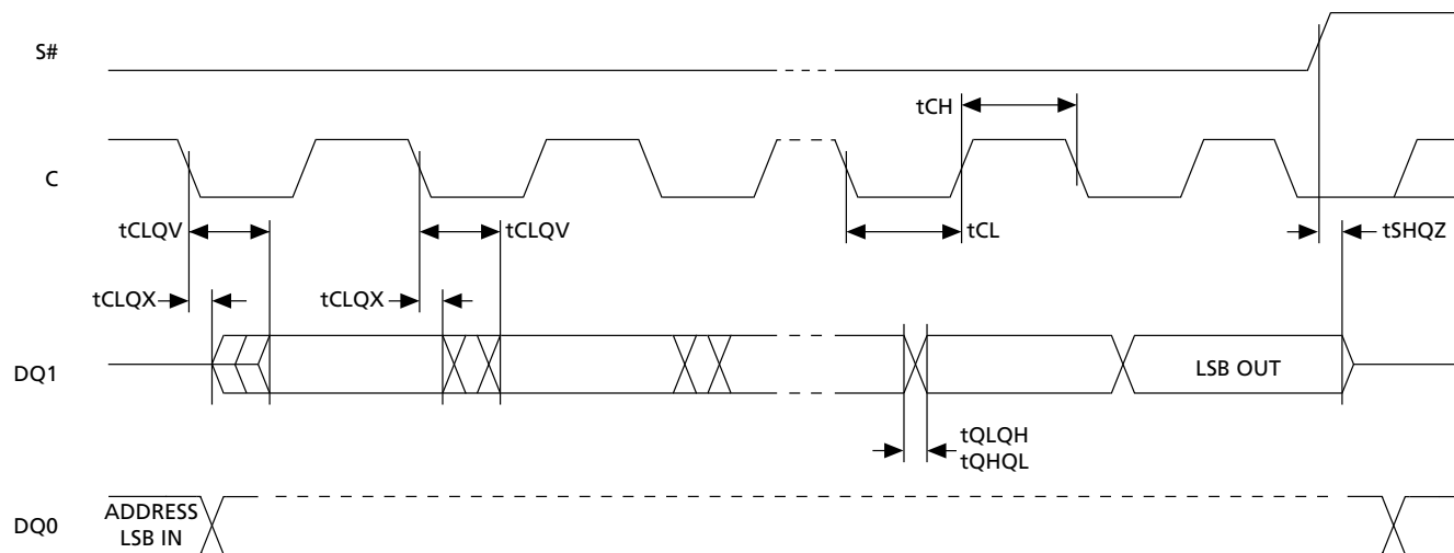
Figure 28: Output Timing
