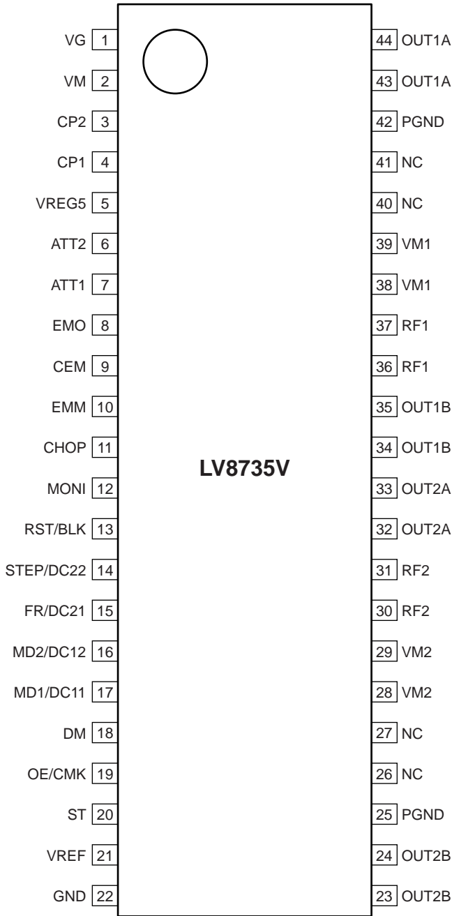
Top view
