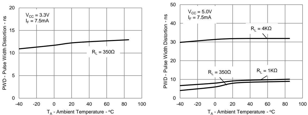
Figure 9: Typical Pulse Width Distortion vs. Ambient Temperature
