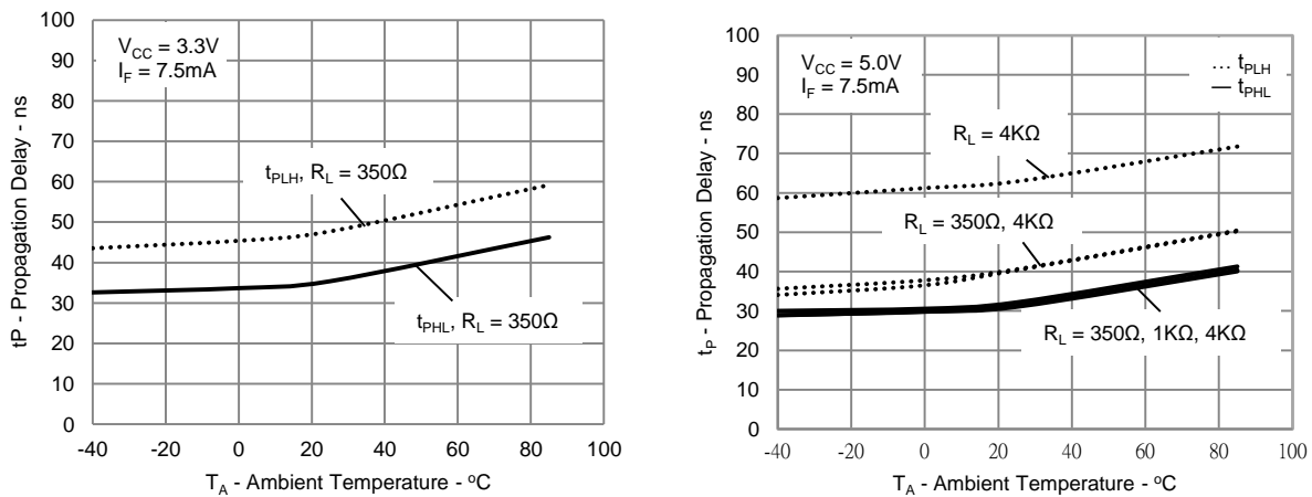
Figure 8: Typical Propagation Delay vs. Ambient Temperature
