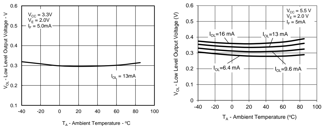
Figure 5: Typical Low Level Output Voltage vs. Ambient
