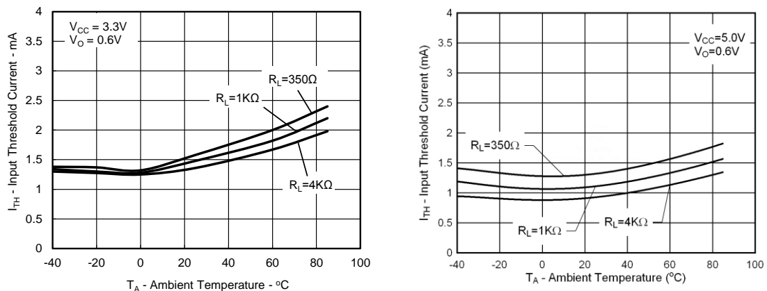
Figure 4: Typical Input Diode Threshold Current vs. Ambient Temperature
