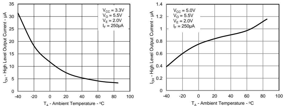
Figure 3: Typical High Level Output Current vs. Ambient Temperature
