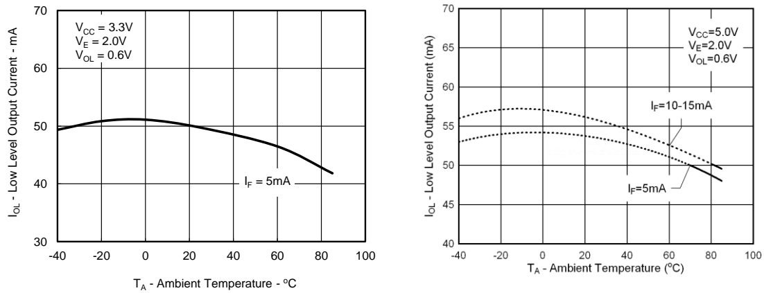
Figure 6: Typical Low Level Output Current vs. temperature
