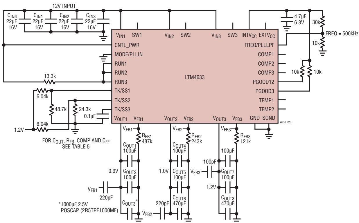
LTM4633 Typical 12V Input to 0.9V at 10A, 1.0V at 10A, 1.2V at 10A with 0.9V and 1.0V Tracking 1.2V
