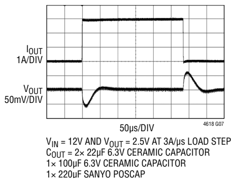
2.5V Transient Response
