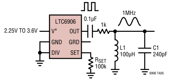
Sine Wave Oscillator
