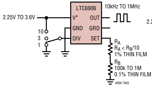
Setting Frequency to 0.1% Resolution with Standard Resistors
