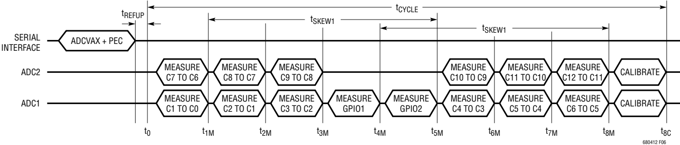
Figure 6. Timing of ADCVAX Command
