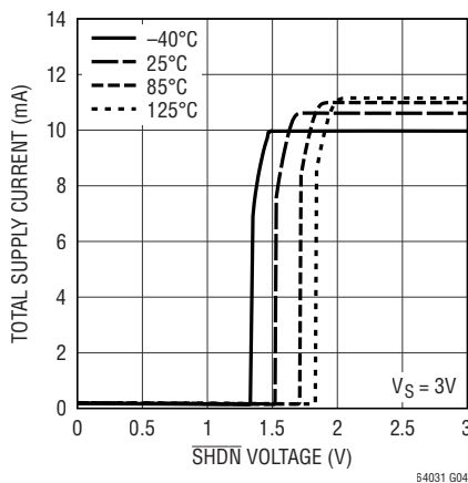
Supply Current vs SHDN Voltage
