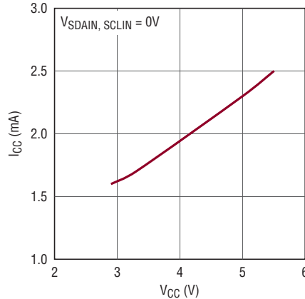
I_{CC} Disabled (ENABLE1-4 Low) Current vs Supply Voltage
