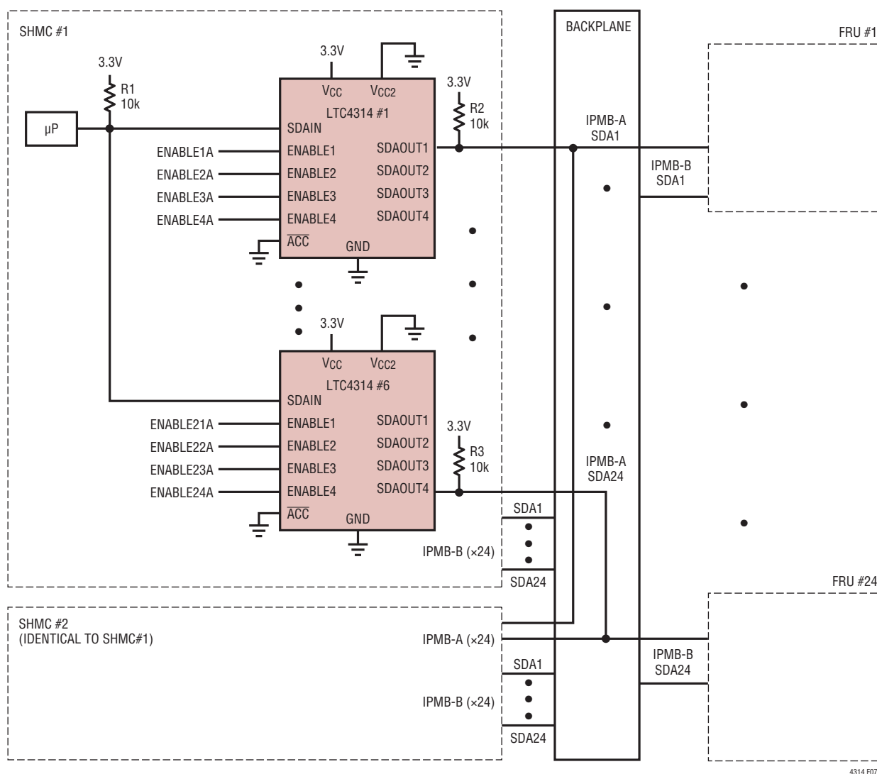
Figure 7. LTC4314s Configured for a Radially Connected Redundant Telecommunications Shelf Manager Application in a 6 × 4 Arrangement. The ENABLE Pins on Only One of the Shelf Managers Are High at Any Time. Only the SDA Path Is Shown for Simplicity
