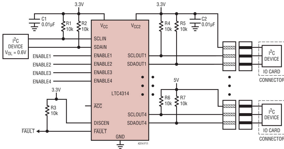
Figure 11. SDA, SCL Hot Swap™ and Operation with a Non-Compliant I²C Device
