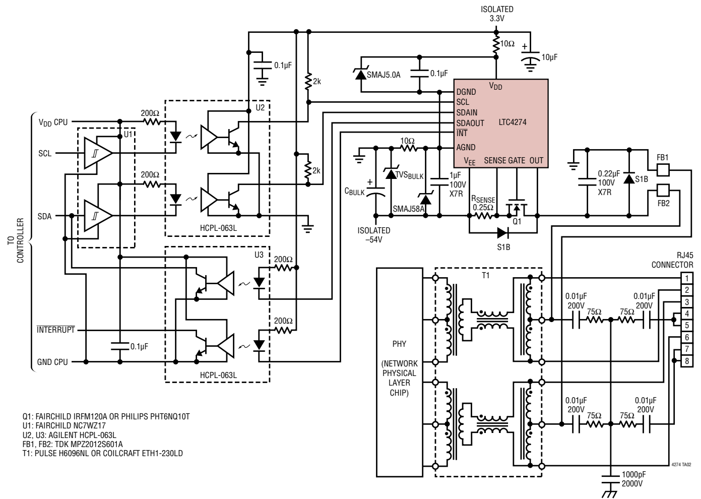
One Complete Isolated Powered Ethernet Port
