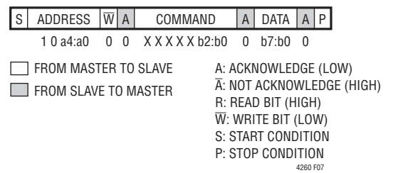
Figure 7. LTC4260 Serial Bus SDA Write Byte Protocol
