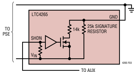
Figure 3. 25k Signature Resistor with Disable
