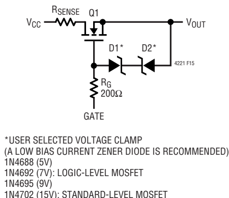
Figure 15. Gate Protection Zener Clamp
