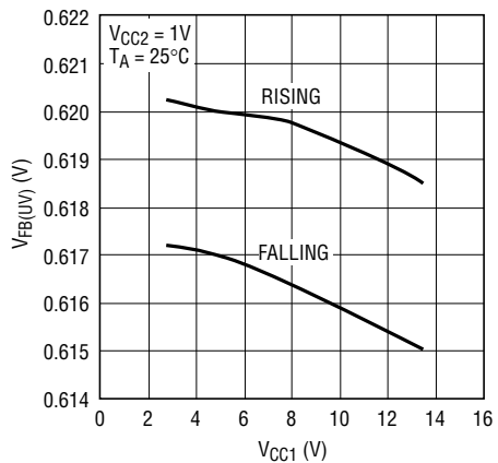
V_{\text{FB(UV)}} vs V_{\text{CC1}}
