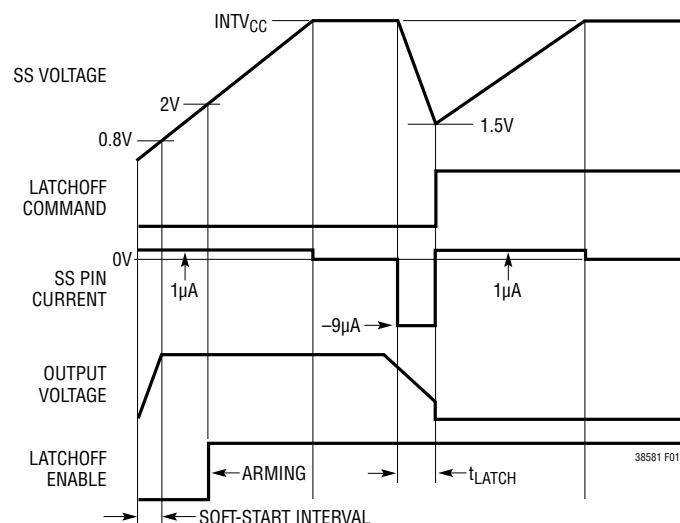
Figure 1. Latchoff Timing Diagram
