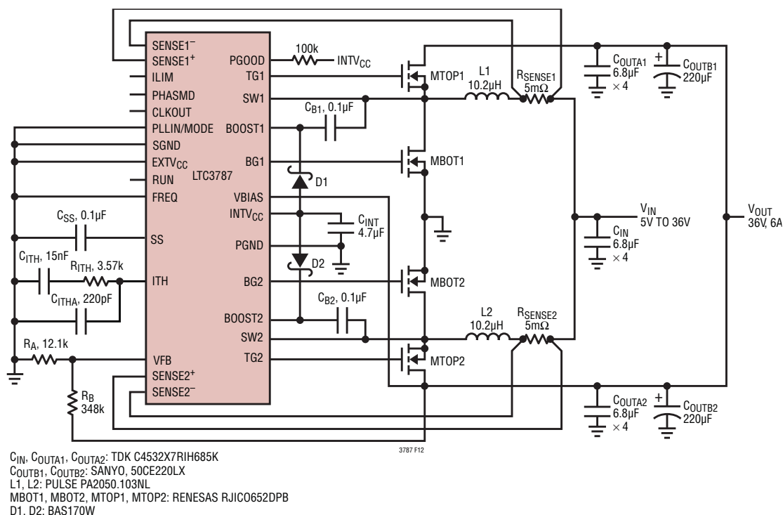
Figure 12. High Efficiency 2-Phase 36V Boost Converter
