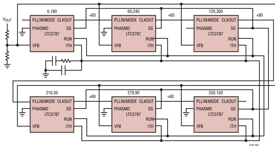
(4d) 12-Phase Operation
