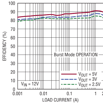
Efficiency vs Load Current in Burst Mode Operation at 2.25MHz
