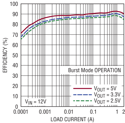
Efficiency vs Load Current at 1MHz
