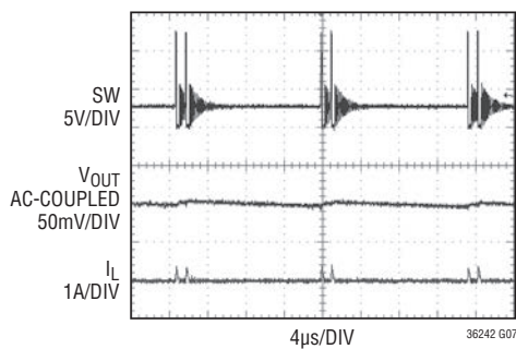
Pulse-Skipping Mode Operation
