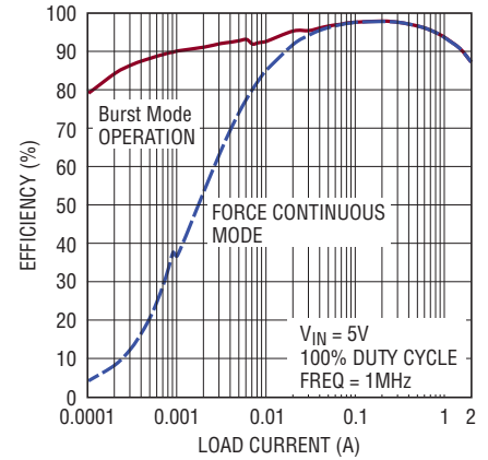
Efficiency vs Load Current in Dropout
