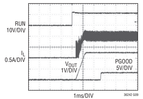
Soft-Start Operation
