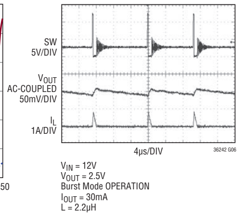
Burst Mode Operation
