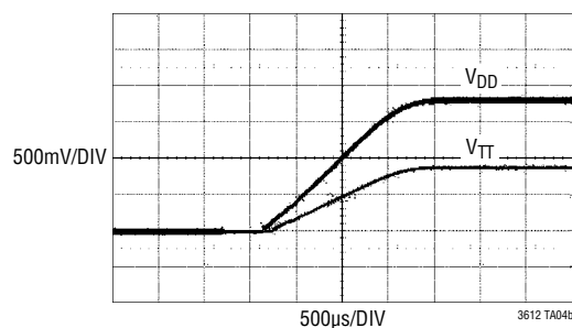
Ratiometric Start-Up
