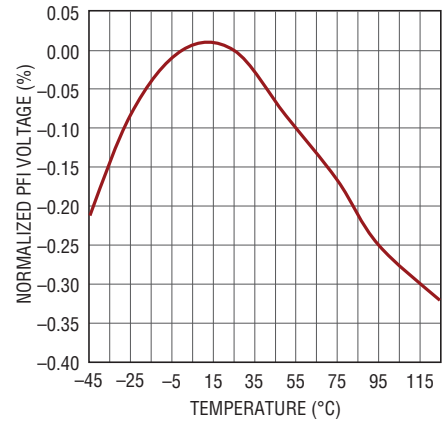
PFI Voltage vs Temperature (Normalized)
