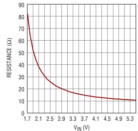
PGOOD Pull Down Resistance vs V_{IN}
