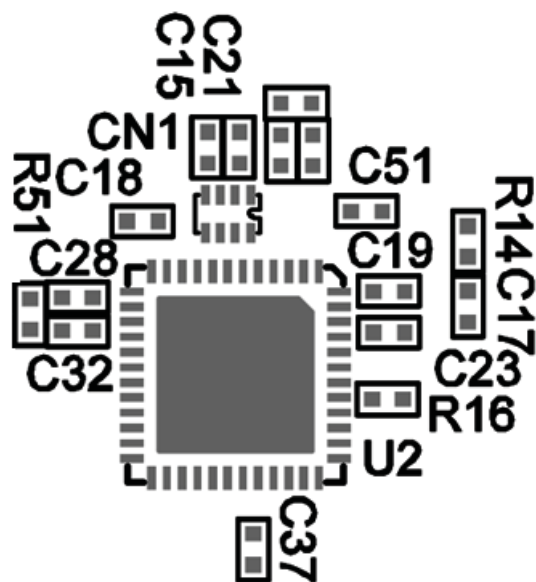
Silkscreen Top
