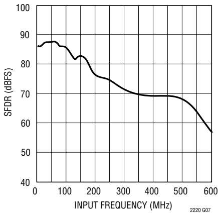
LTC2220-1: SFDR (HD2 and HD3) vs Input Frequency, -1dB, 1V Range, LVDS Mode
