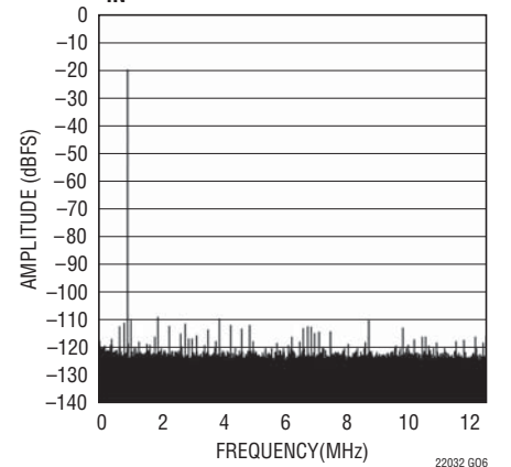
LTC2203: 128K Point FFT, f_{IN} = 1\text{MHz} , -20\text{dBFS} , \text{PGA} = 0
