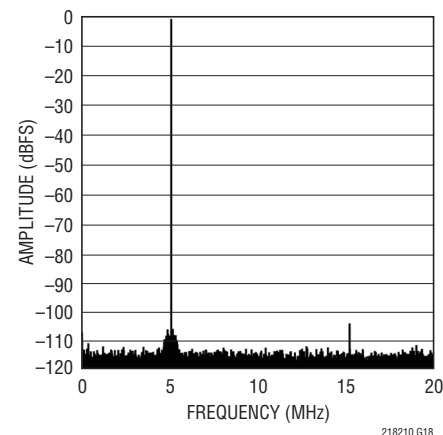
LTC2181: 64k Point FFT, f_{IN} = 5\text{MHz} , -1dBFS, 40Mps
