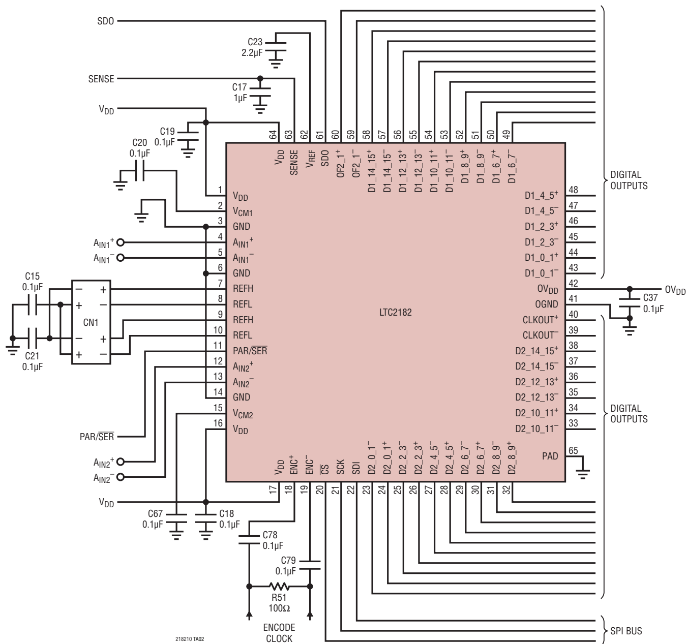
LTC2182 Schematic
