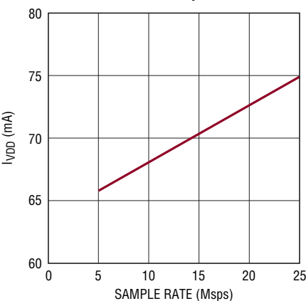
LTC2170-14: I_{VDD} vs Sample Rate, 5MHz Sine Wave Input, -1dBFS
