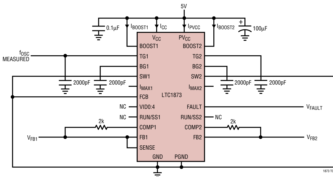
Test Circuit 1
