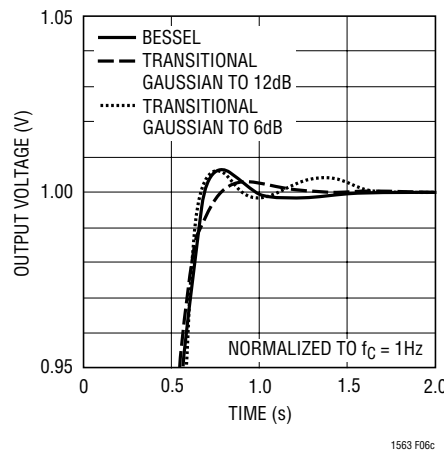
Figure 6c. Step Response—Settling
