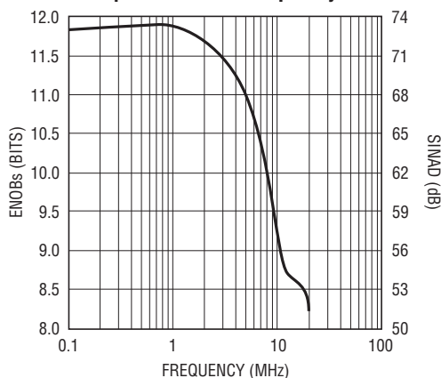
ENOBs and SINAD vs Input Sinewave Frequency
