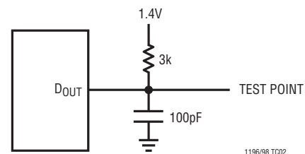
Load Circuit for t dD0 , t r and t f
