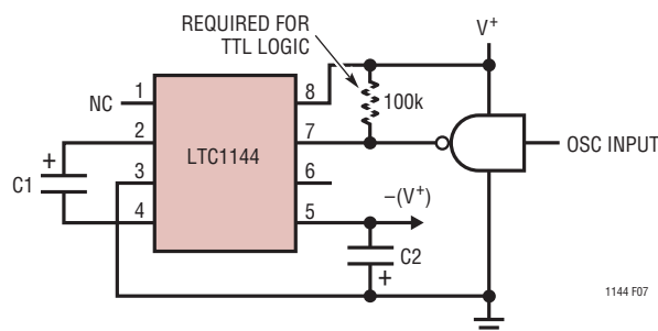
Figure 7. External Clocking
