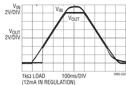
Dropout Performance
