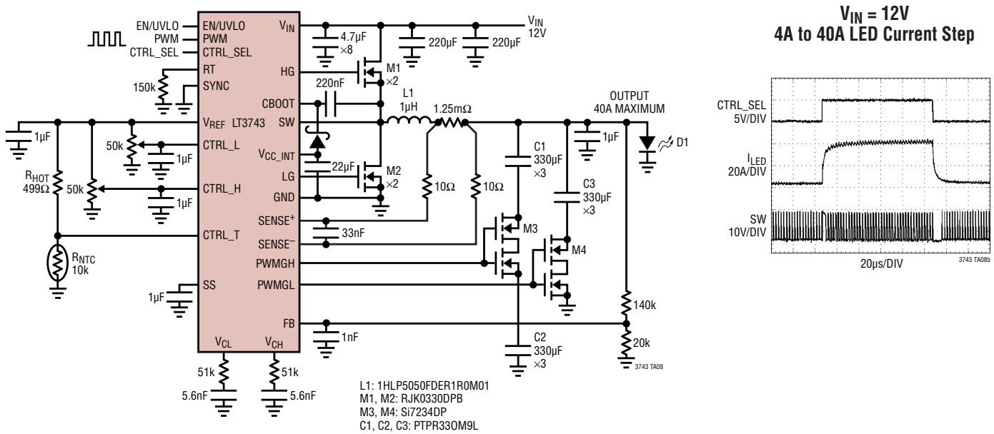
12V, 40A Pulsed LED Driver
