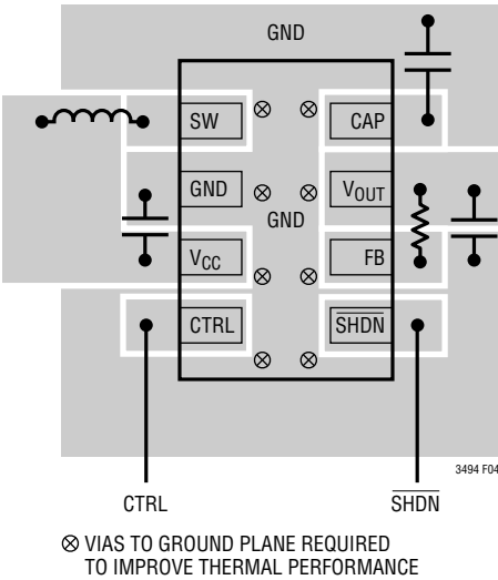
Figure 4. Recommended Layout
